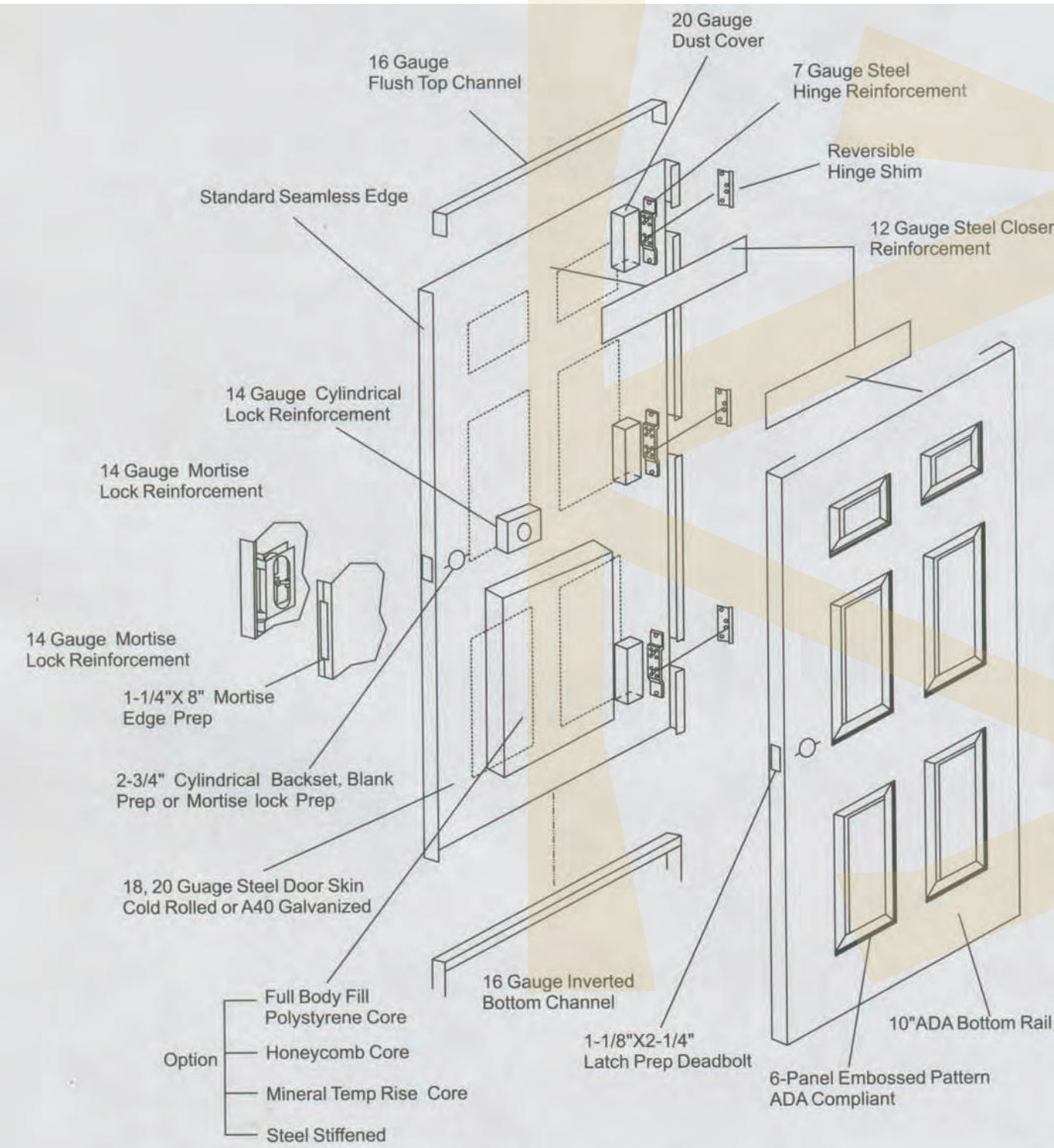
USA FIRE-RATED DOOR LEAF STRUCTURE
