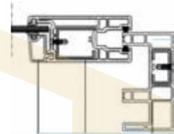
Multi-Chamber structure
