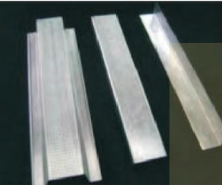
Furring channel & main channel
