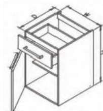
■单抽单门地柜 Base cabinet 1 door 1 drawer
