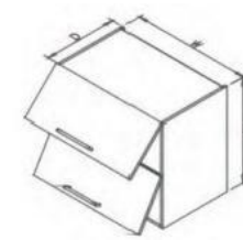
■双门上翻门吊柜 Wall lift-up cabinet 2 doors
