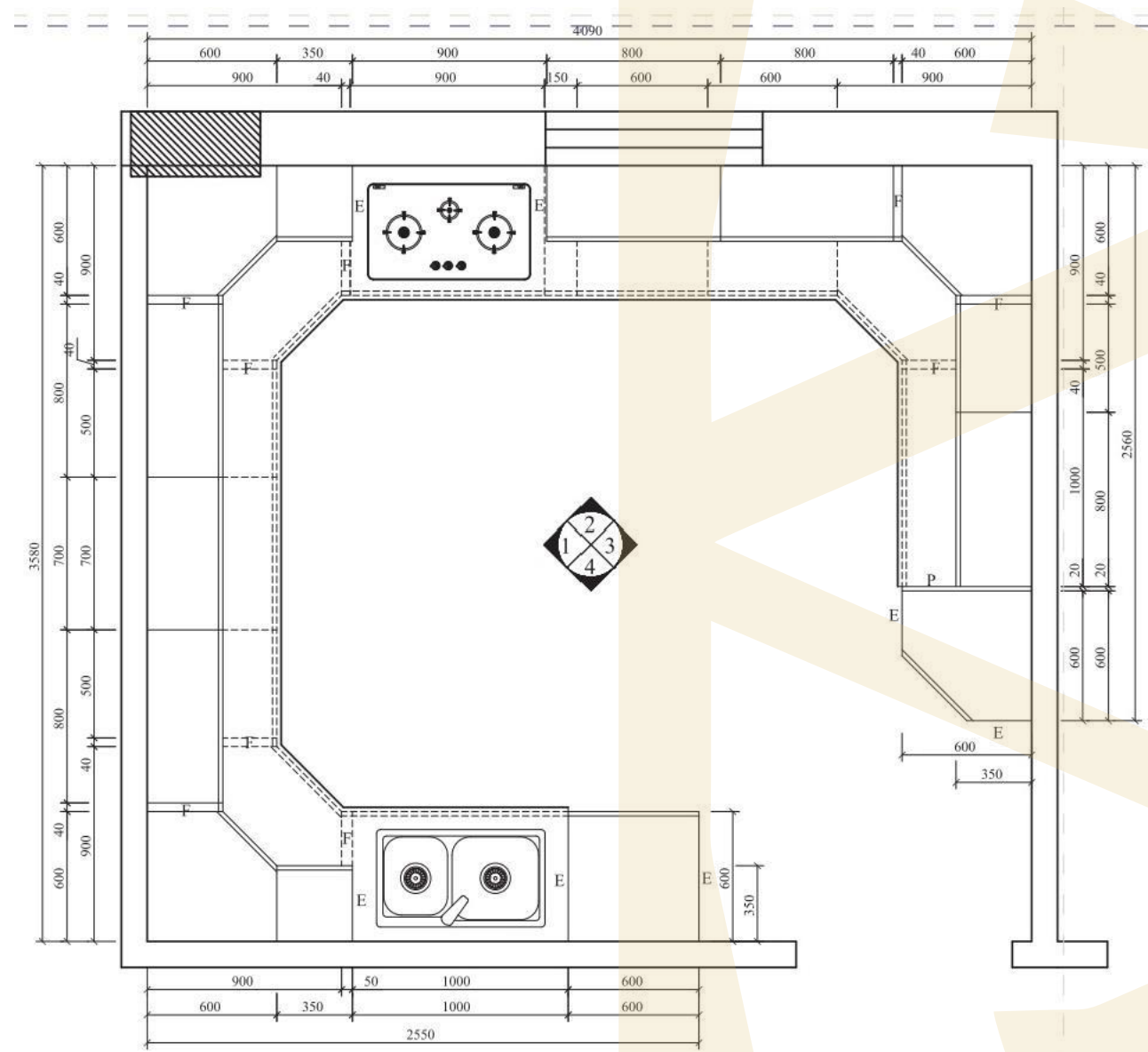
MAIN KITCHEN PLAN
