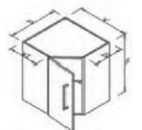
■单门平开转角地柜 Base diagonal cabinet 1 door
