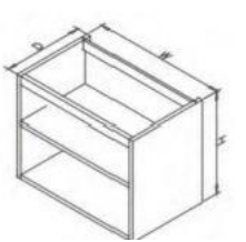
■开方层板柜-1片活动层板 Open shelf cabinet 1 shelf
