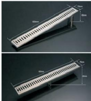
FD-6385 Floor Drainer
