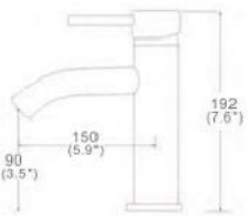
FT-8131C-UPC FT-8131B-UPC Single Handle Basin Faucet Tall Type Available
