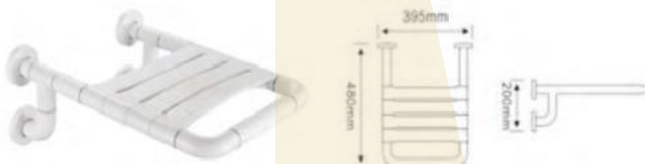
BAS-416 Handrail
