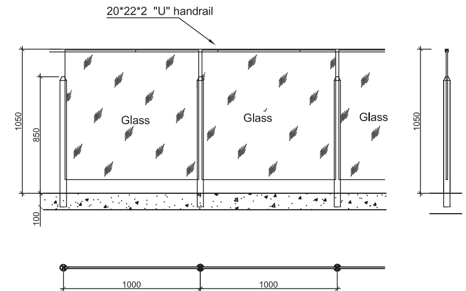
Railing Elevation 护栏立面图
