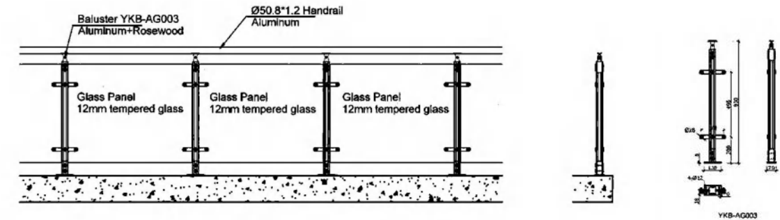
Railing Elevation 护栏立面图
