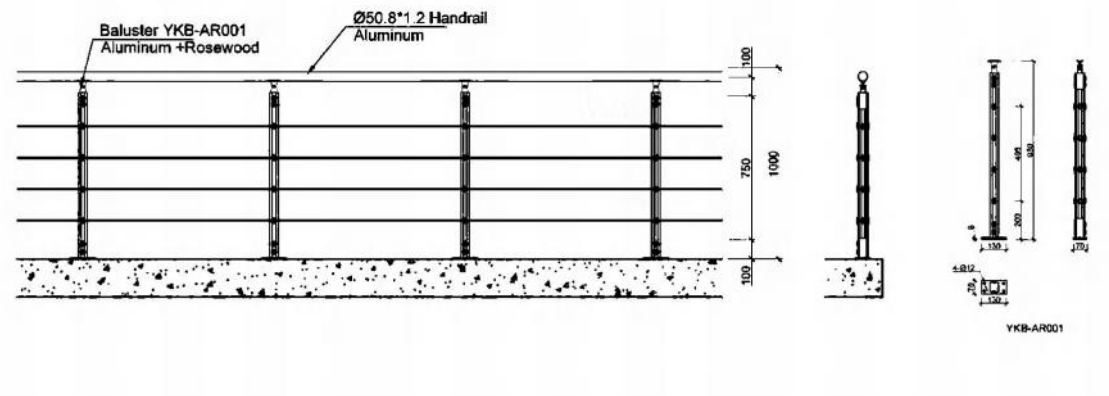
Railing Elevation 护栏立面图
