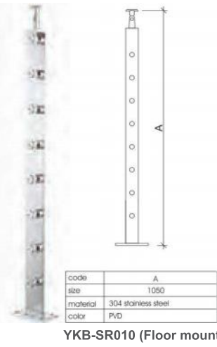
YKB-SR010 (Floor mounted)
