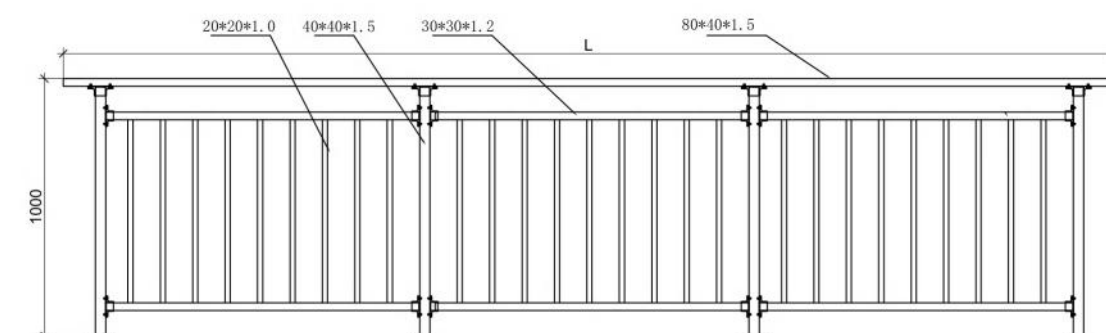
Railing Elevation 护栏立面图
