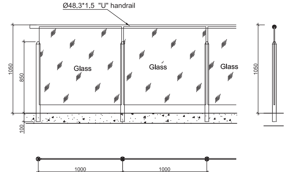
Railing Elevation 护栏立面图
