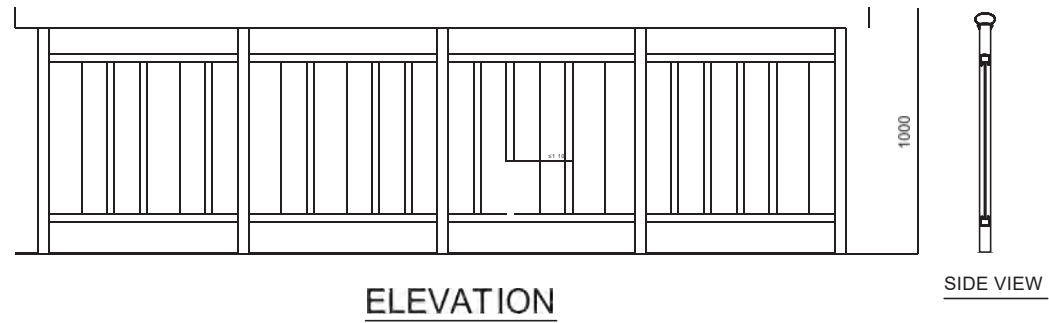
Railing Elevation 护栏立面图
