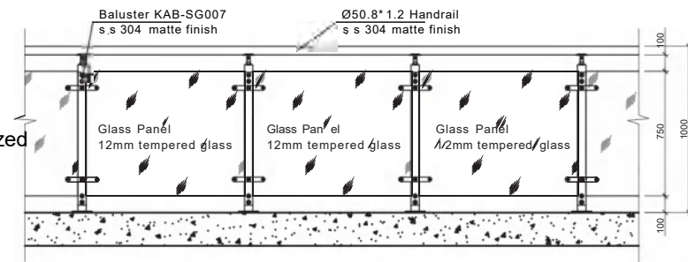
Railing Elevation 护栏立面图
