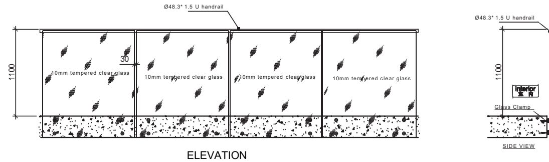
Railing Elevation 护栏立面图
