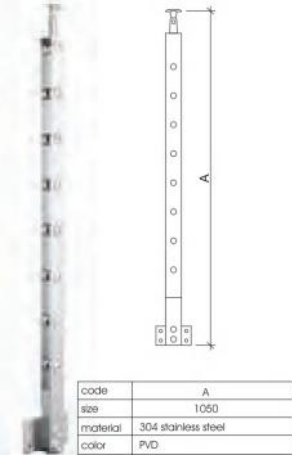
YKB-SR010 (Wall mounted)
