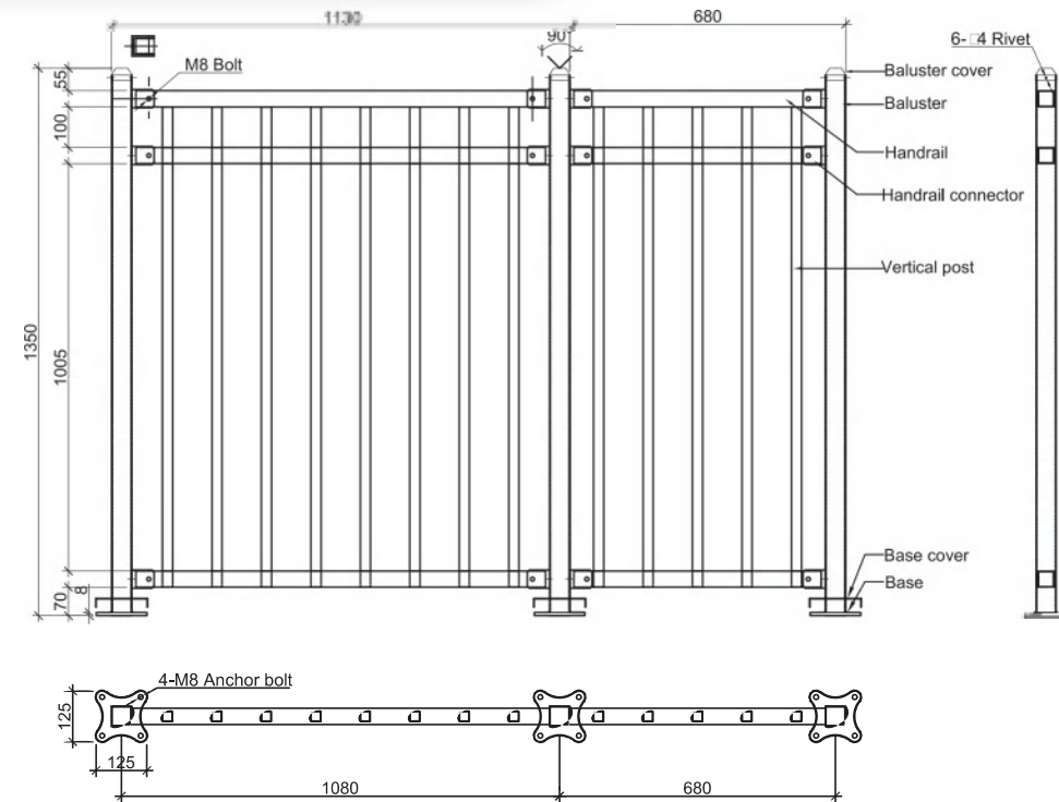
Railing Elevation 护栏立面图
