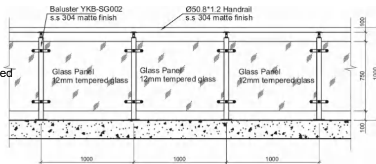
Railing Elevation 护栏立面图
