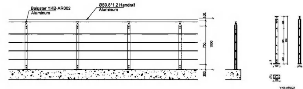
Railing Elevation 护栏立面图
