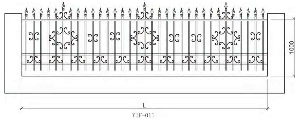
Railing Elevation 护栏立面图
