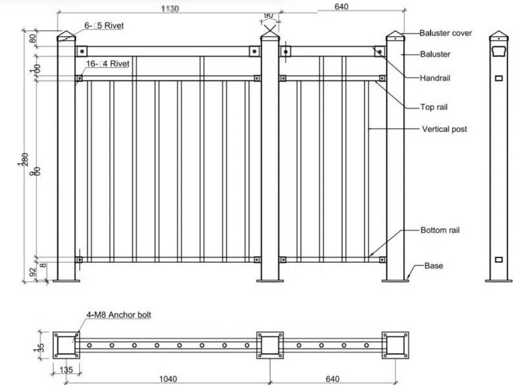
Railing Elevation 护栏立面图
