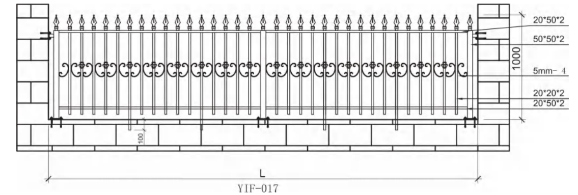
Railing Elevation 护栏立面图
