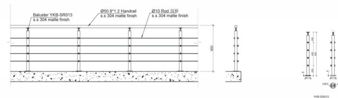
Railing Elevation 护栏立面图
