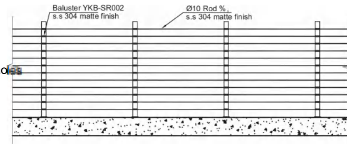
Railing Elevation 护栏立面图
