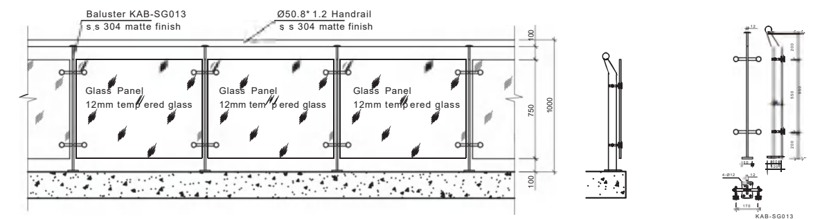
Railing Elevation 护栏立面图
