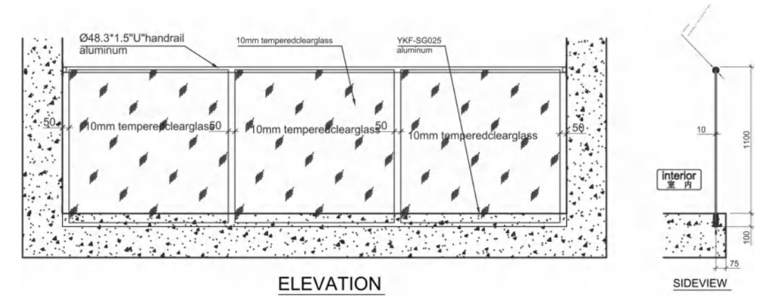
Railing Elevation 护栏立面图
