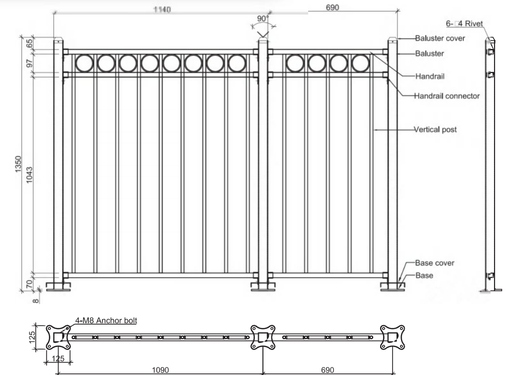
Railing Elevation 护栏立面图
