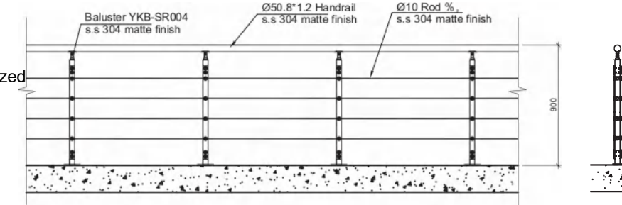
Railing Elevation 护栏立面图
