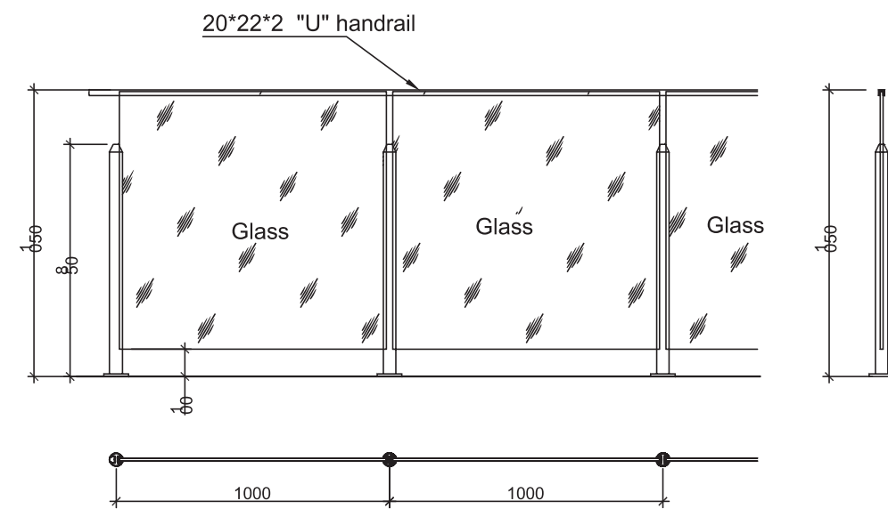
Railing Elevation 护栏立面图
