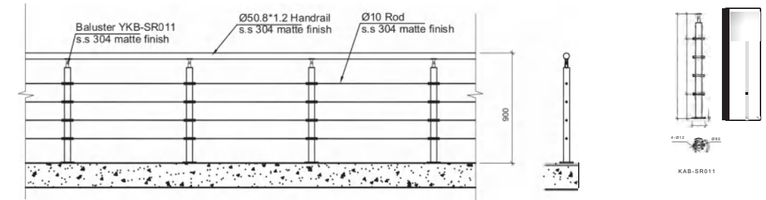
Railing Elevation 护栏立面图
