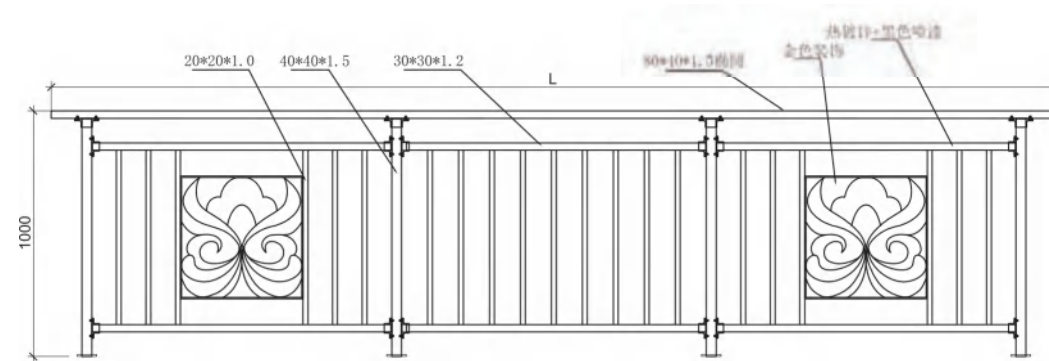
Railing Elevation 护栏立面图
