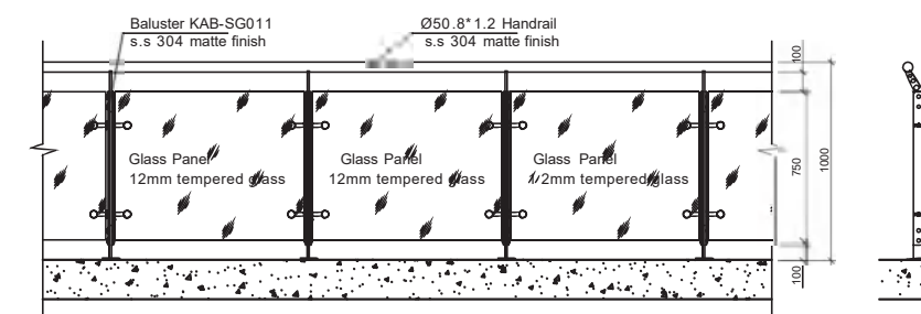
Railing Elevation 护栏立面图
